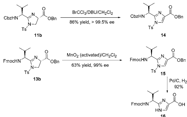
Scheme 2. Synthesis of Imidazole-Based Protected Amino Acids
