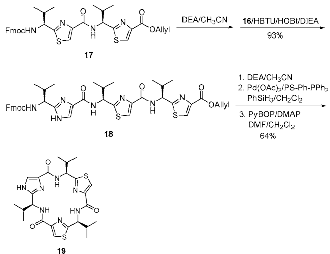
Scheme 3. Incorporation of Imidazole-Based Amino Acid 16 into a Macrolactam Analogue of Bistratamide H ( 19 ) 6k
